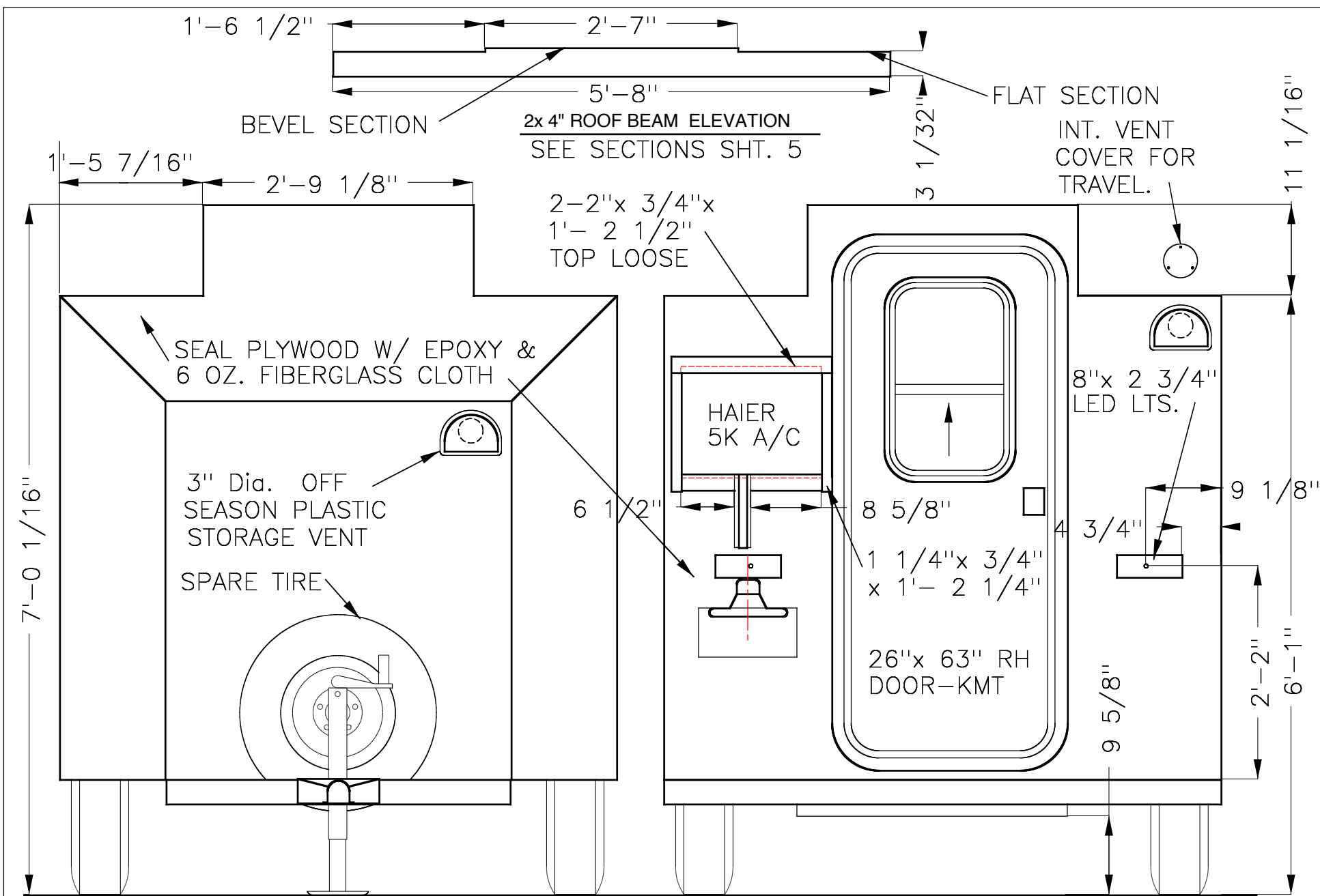
FRONT ELEVATION
