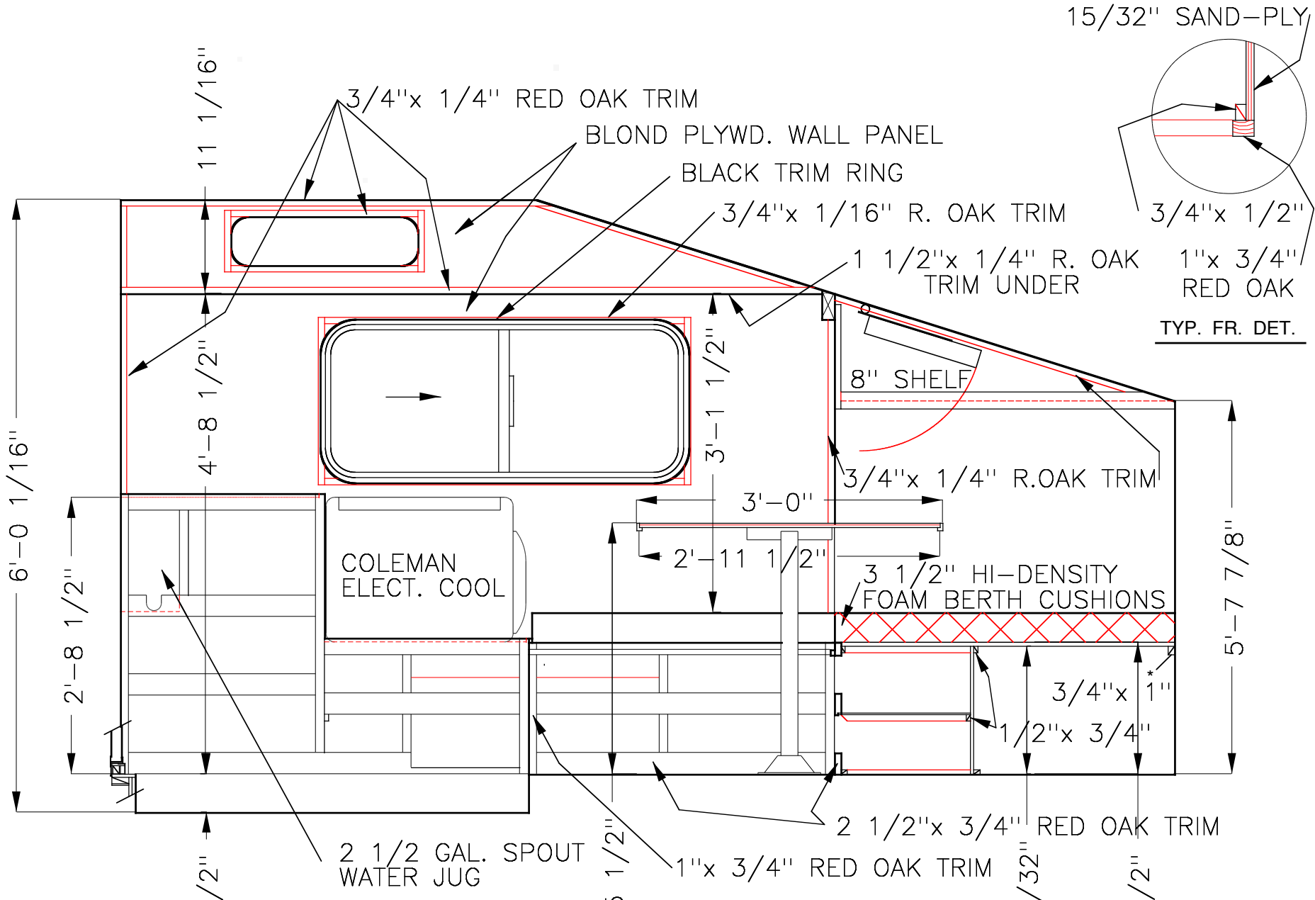
LEFT INT. ELEVATION
